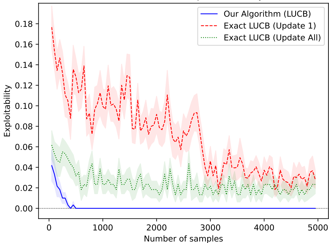
Kuhn Poker, Exact Computation, Player o
